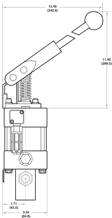
Left View
